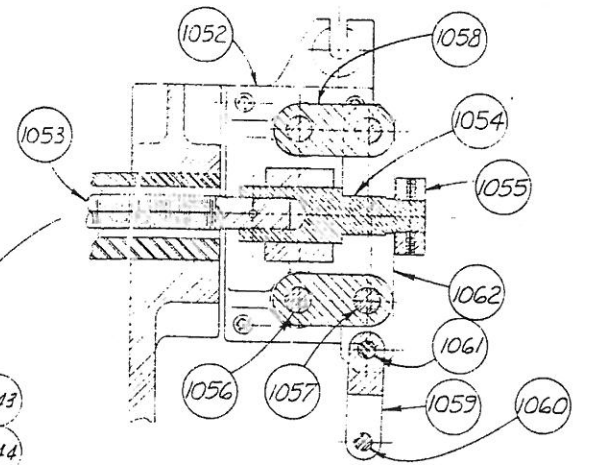
SECTION THRU STOCK GAUGE RELIEF MECHANISM (ALSO SEE 3WH-1131)
