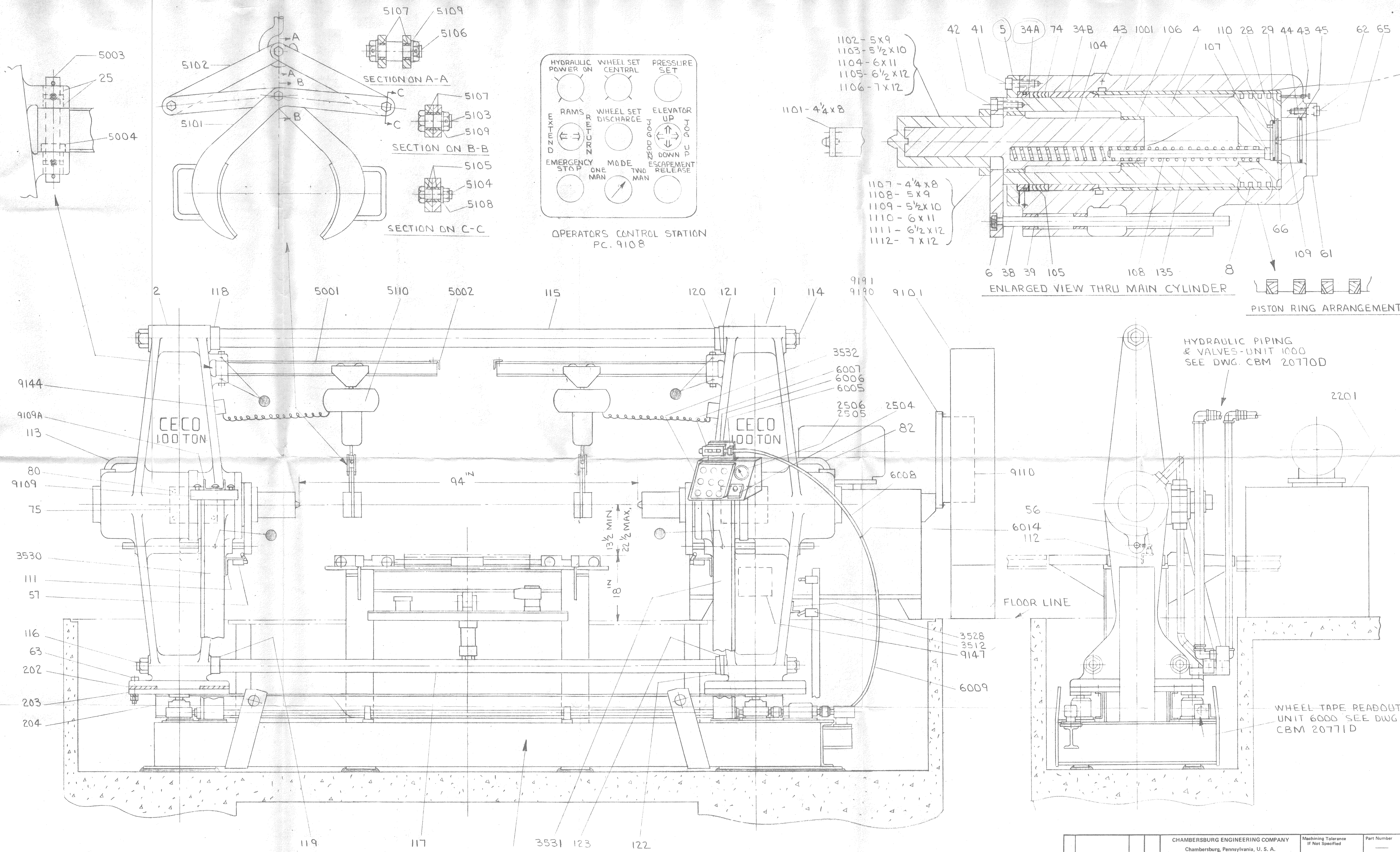
ELEVATOR UNIT 3500 SEE DWG. CBM 20771D
