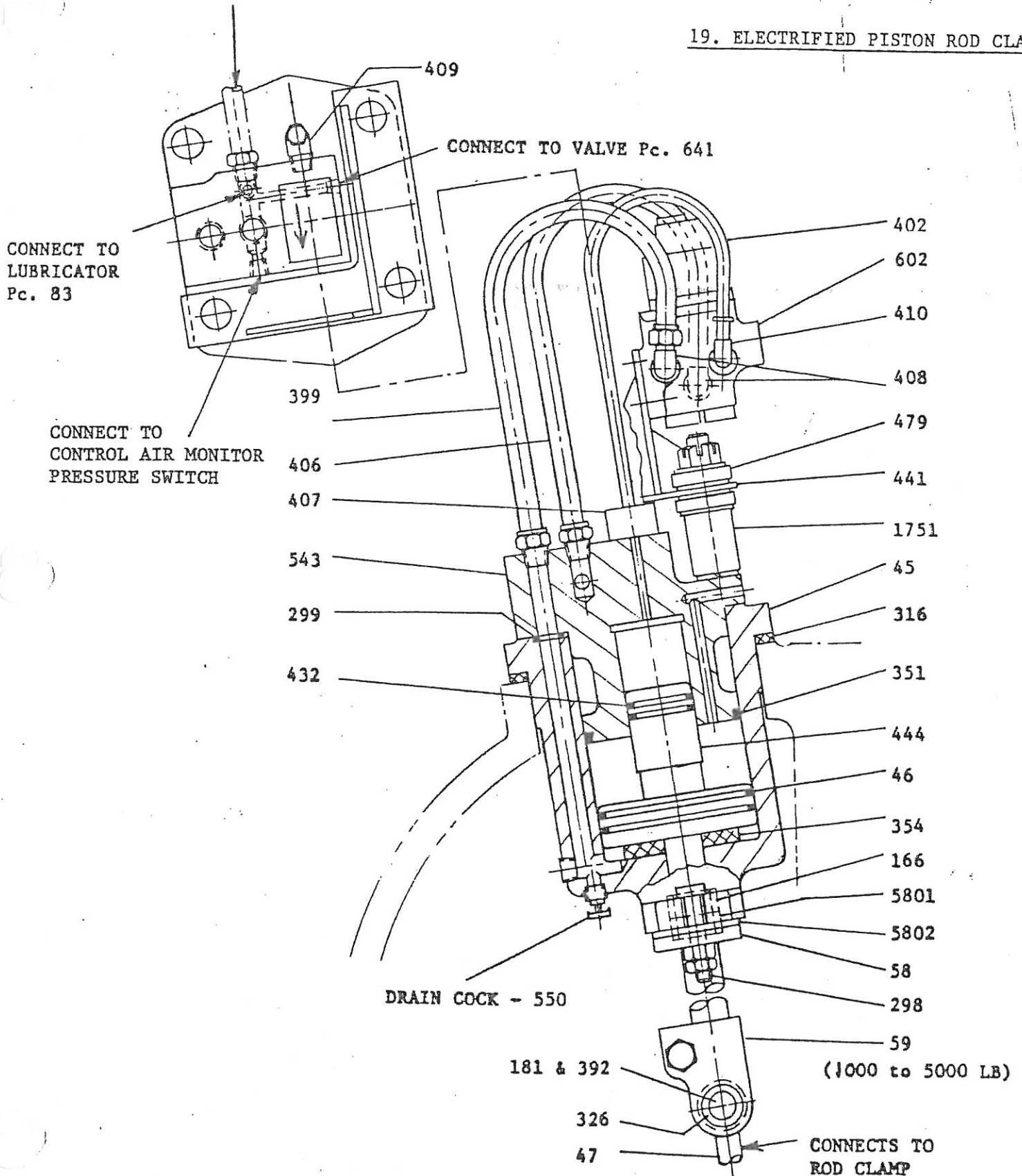
DOUBLE ACTING CLAMP CYLINDER ARRANGEMENT
