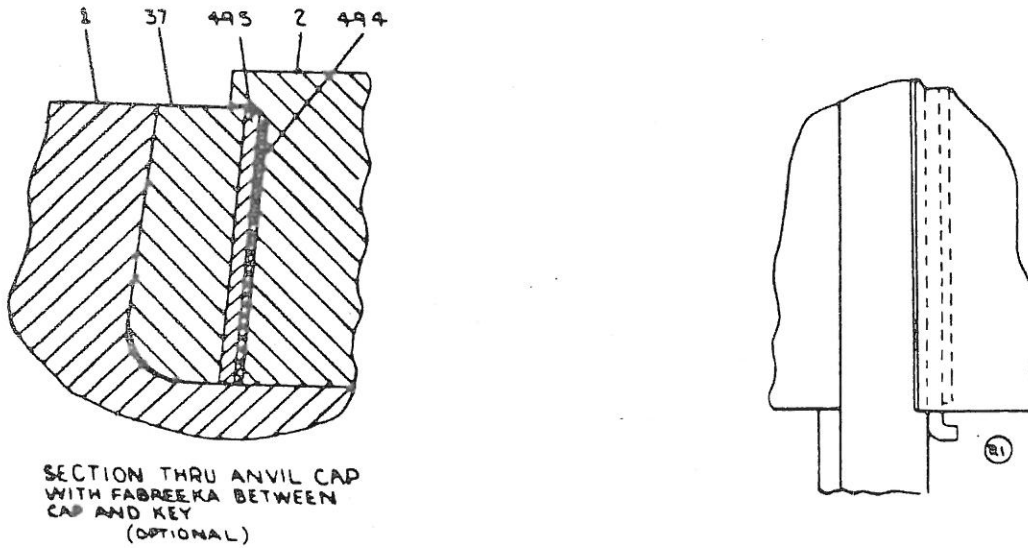
ANVIL CAP KEY FABREEKA PAD ASSEMBLY
