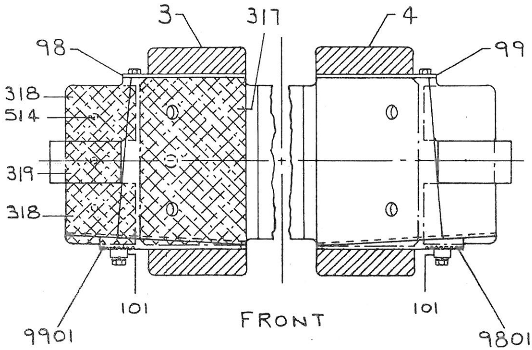
SPECIAL TAPERED FRONT WEARING PLATES, 9801 AND 9901 AND COMPOSITION LINERS (OPTIONAL FEATURES)
