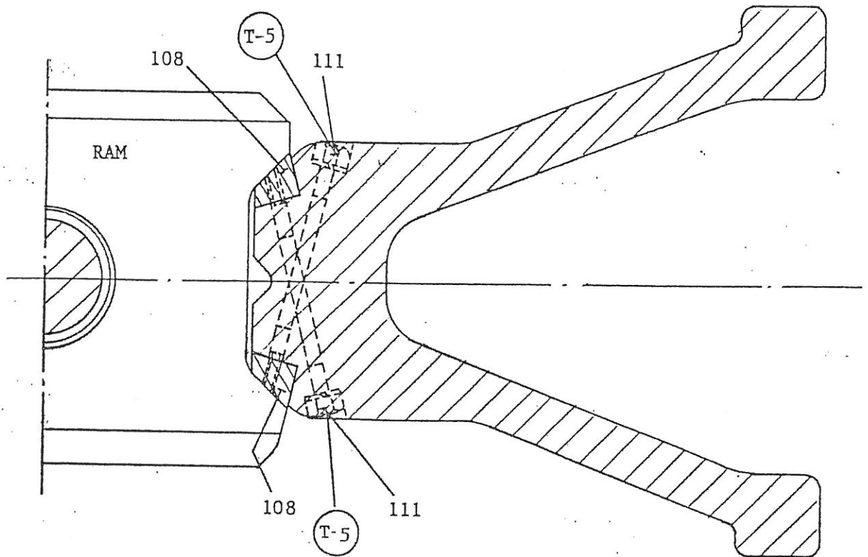
SECTION THRU RAM GUIDES
