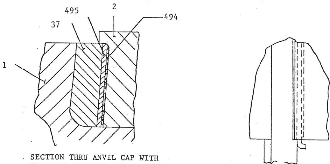
Special Tapered Wearing Wedge Arrangement
