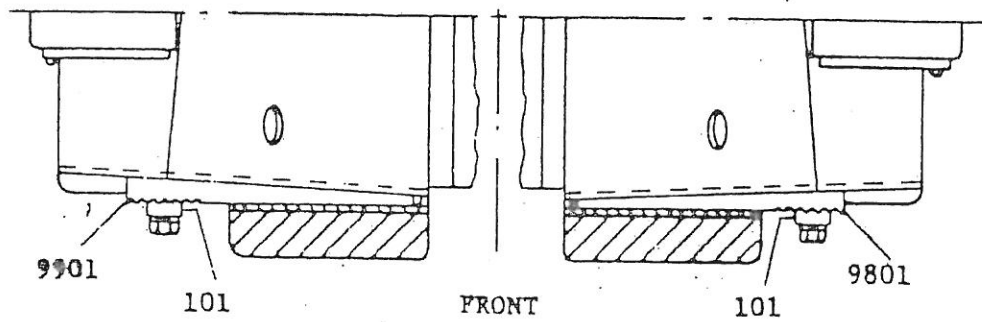
Special Tapered Wearing Wedge Arrangement
