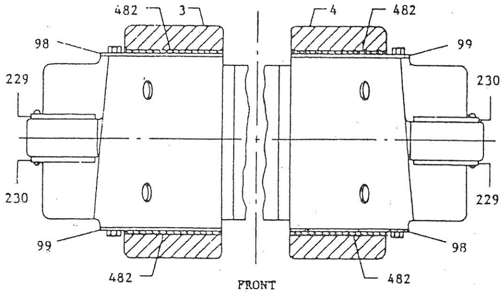
Standard Wearing Plate Arrangement
