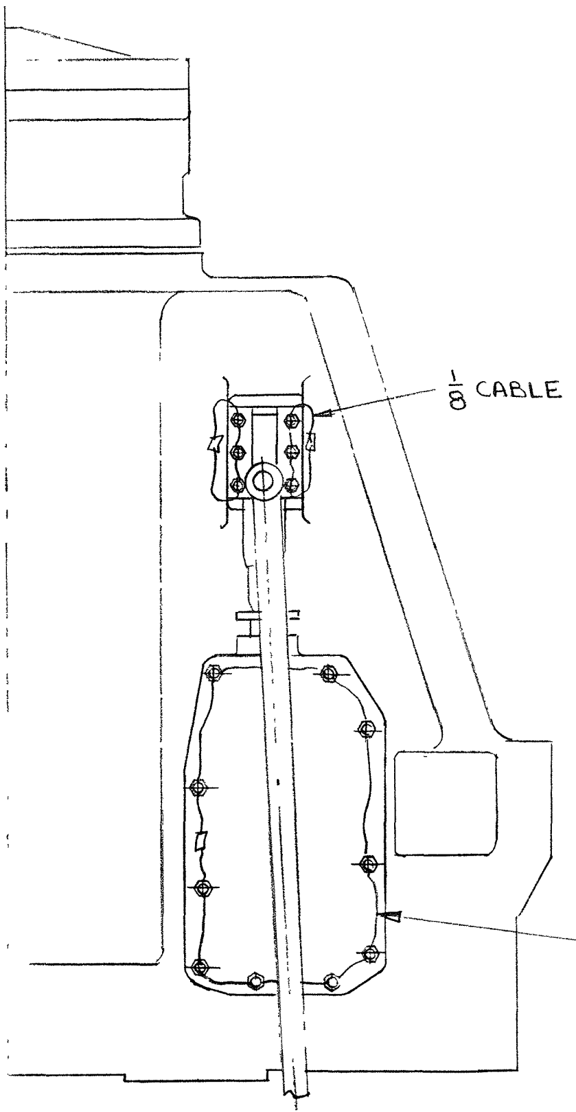
VIEW OF FLAT VALVE CYLINDER SAFETY WIRING
