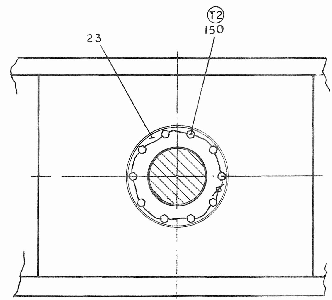
SECTION ON A-A BOTTOM VIEW OF CROWN
